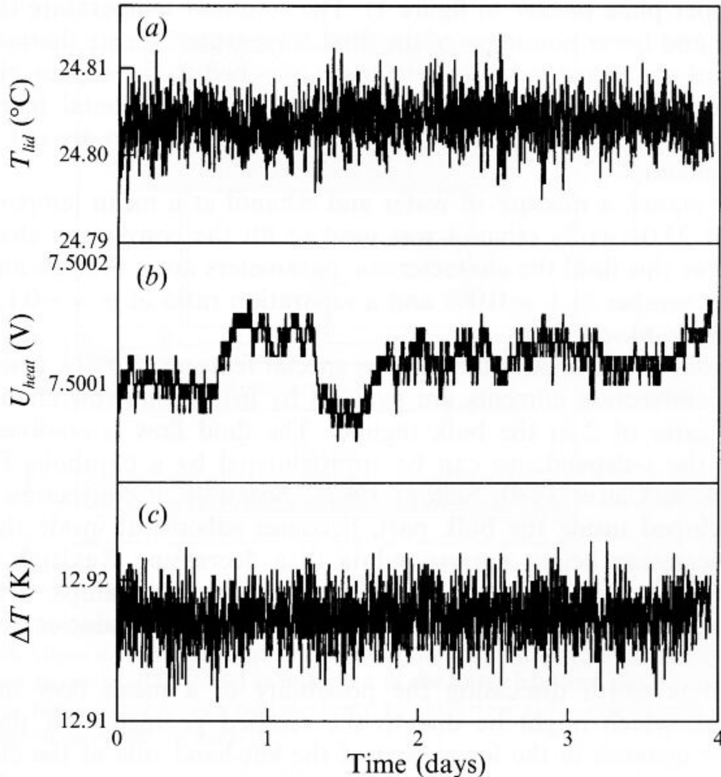
FIGURE 2. Long-time stability of the important externally controlled parameters applied to the convection cell. Shown as functions of time for about four days are (a) the temperature of the lid of the aluminium box, (b) the voltage used for heating from below, and (c) the temperature difference between the top and bottom boundaries of the fluid.
