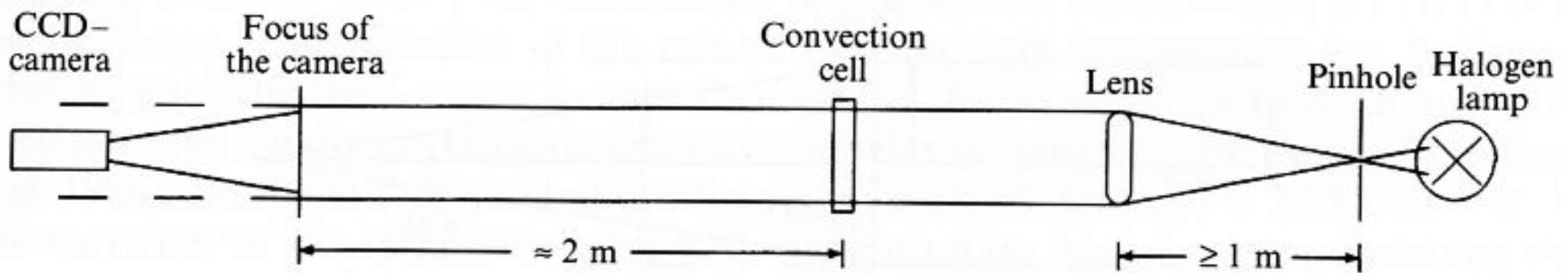
FIGURE 3. Schematical sketch of the optical setup. White light coming from a halogen lamp is made weakly convergent by means of a lens and illuminates the convection channel from the front side ( x, z -plane). The resulting images taken by the CCD-camera are further processed using frame-grabbing facilities implemented in a PC/AT-computer (not shown here).
