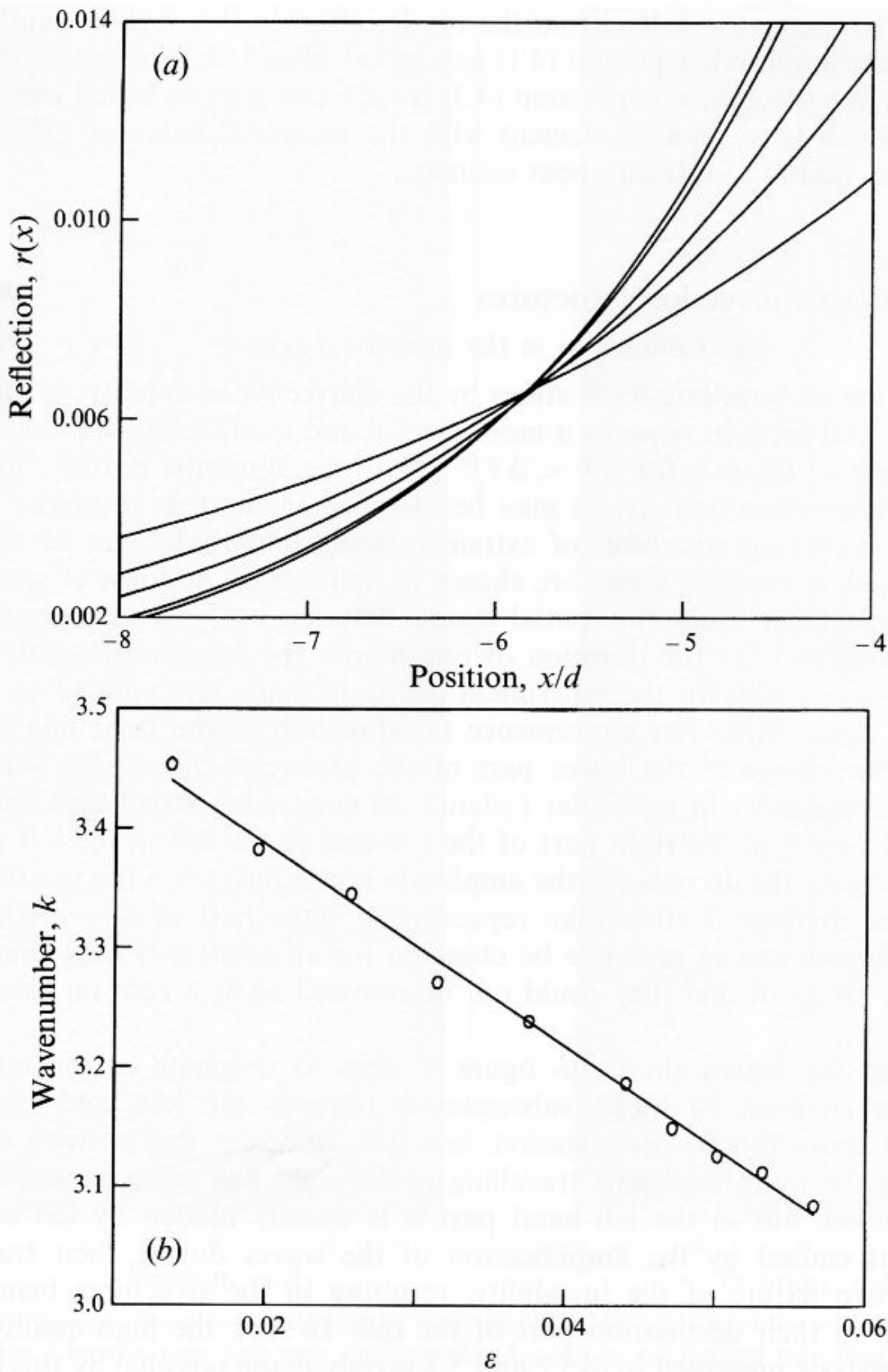
FIGURE 8. Results obtained from the periodic heat pulse measurements through fits analogous to that shown in figure 7(b). (a) The function r(x) = (B_0/A_0) \exp(2\varepsilon x/v_g \tau_0) is plotted for different values of the temperature difference. The lines intersect at the centre of reflection at x \approx -6d determining the reflection coefficient as r \approx 0.006 . (b) The wavenumber as a function of \varepsilon extracted from the measurements (open circles) can be modelled by the straight line obeying the law k(\varepsilon) = k_c - (c_0 \varepsilon/v_g \tau_0) . This yields a critical wavenumber of k_c = 3.56 and c_0/v_g \tau_0 = 8.46 .
