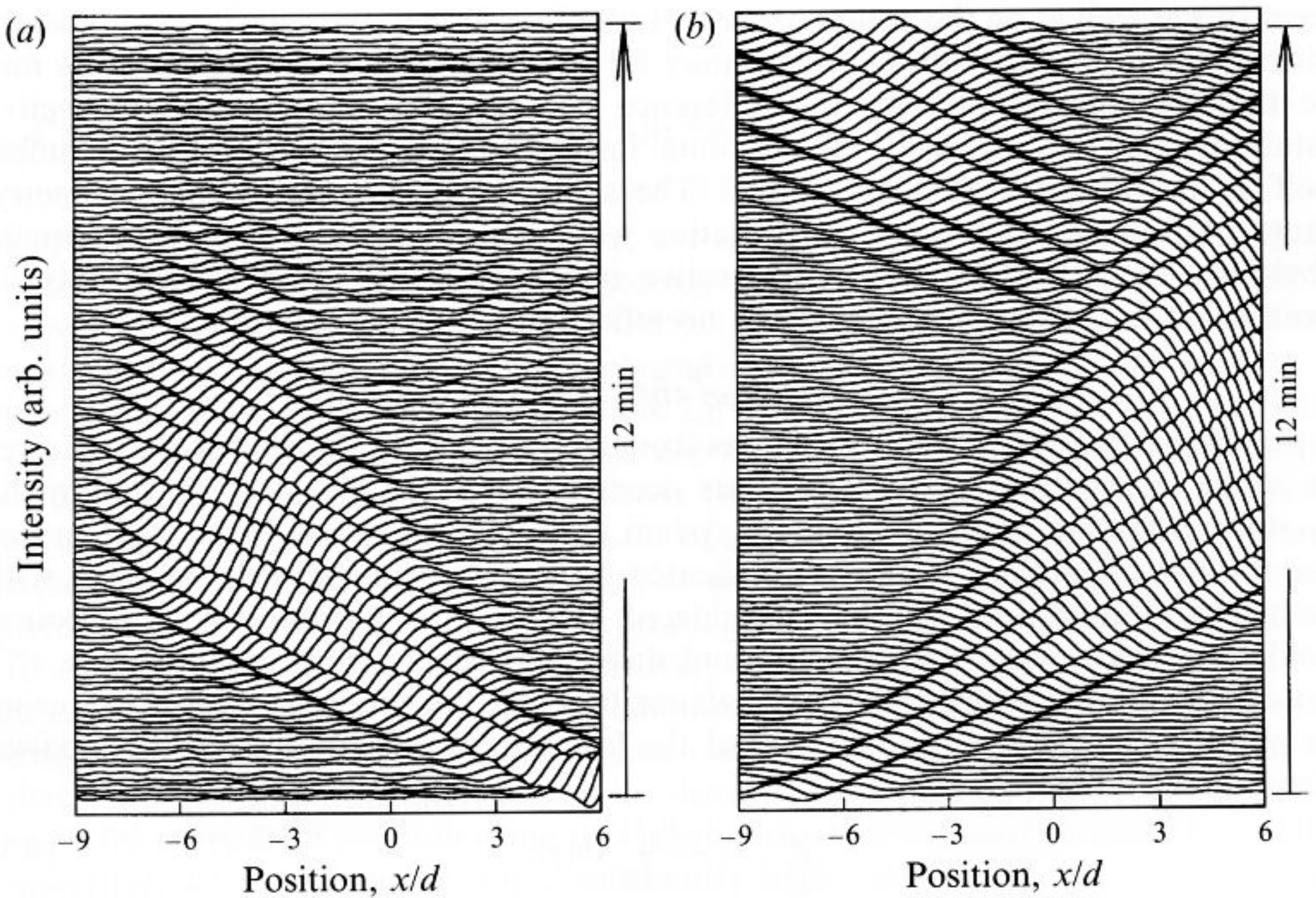
FIGURE 6. Space-time plot to demonstrate the reflection behaviour of the convection channel. For this sort of representation several profile lines taken consecutively in time are plotted one above the preceding one (here for a duration of 12 minutes altogether). A voltage pulse applied to the resistor shown in figure 1 generates a localized disturbance which penetrates through the channel. The measurements correspond to convectively but not absolutely unstable situations ( \varepsilon = 0.03 ). The resistor for generating the heat pulse is located outside the plotted area on the right-hand on (a) and on the left-hand side on (b). (a) Convection cell used in our experiments as shown in figure 1 and explained in detail in the text with the homogeneous region extending between x = \pm 3d . A very weak reflected wave can be seen in the upper right part of the picture. (b) Rectangular convection cell similar to the one described in figure 1, but without ramps and instead the bulk part extended over the entire lateral dimension. Now the wave reflected from the right-hand boundary can clearly be recognized.
