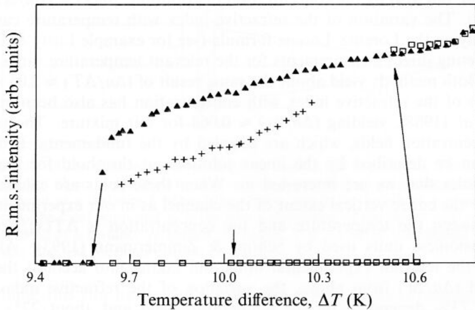
FIGURE 5. Stability diagram as measured for our working fluid. The r.m.s. -intensity \bar{I}_{rms} of the respective profile lines is shown as a function of the applied temperature difference \Delta T with open squares corresponding to increasing and closed triangles to decreasing \Delta T . The onset of nonlinear convection for \Delta T_c = 10.61 K is clearly visible. When reducing the temperature difference, convection does not vanish until the lower value of \Delta T_s = 9.61 K is reached, which is caused by the subcritical nature of the bifurcation leading to the observed hysteresis. The small arrow at \Delta T_c^{con} = 10.03 K indicates the onset of the convective instability, where the growth rate of a homogeneous disturbance is zero ( \varepsilon = 0 ). The crosses inside the stability diagram correspond to stable localized travelling waves (confined states).
