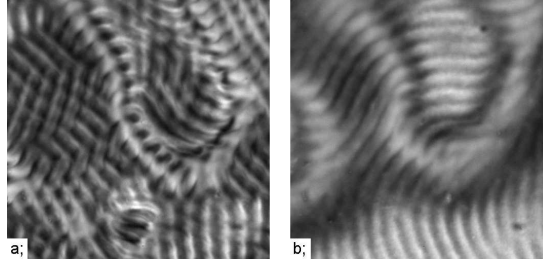
Figure 15. Snapshots of nonstandard electroconvection pattern in case H taken with crossed polarizers. a; oblique rolls, b; parallel rolls.
