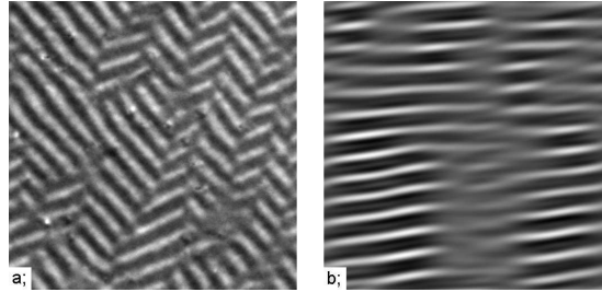
Figure 14. Snapshots of nonstandard electroconvection pattern in case G taken with crossed polarizers. a; oblique rolls, b; parallel rolls. Contrast was enhanced by digital processing. The initial director orientation is horizontal.
