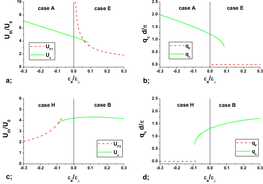
Figure 2. Threshold voltage U_{th}/U_0 and the critical wavenumber q_c versus the dimensionless dielectric anisotropy \epsilon_a/\epsilon_{\perp} calculated from Eqs. 7 and 8. (a,b): Planar alignment with \sigma_a > 0 ; (c,d): homeotropic alignment with \sigma_a < 0 . Dashed lines correspond to the Fredericksz transition, solid lines to the direct EC transition.
