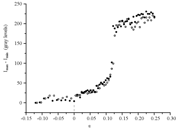
Figure 12. Voltage dependence of the contrast of the EC pattern in case D . \varepsilon = (U^2 - U_c^2)/U_c^2 is a dimensionless control parameter. Contrast is defined as the difference of the maximum I_{max} and minimum I_{min} intensities within the pattern.
