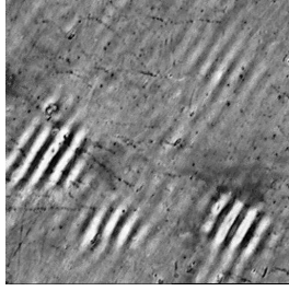
Figure 11. Snapshot of EC pattern in the Freedericksz distorted planar geometry of case D .
