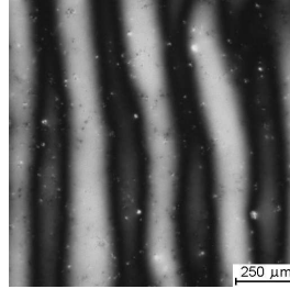
Figure 13. The prewavy pattern in homeotropic MBBA. d = 50\mu\text{m} .
