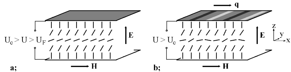
Figure 8. Director orientation in case C. a; Fredericksz distorted state, b; with superposed electroconvection pattern.
