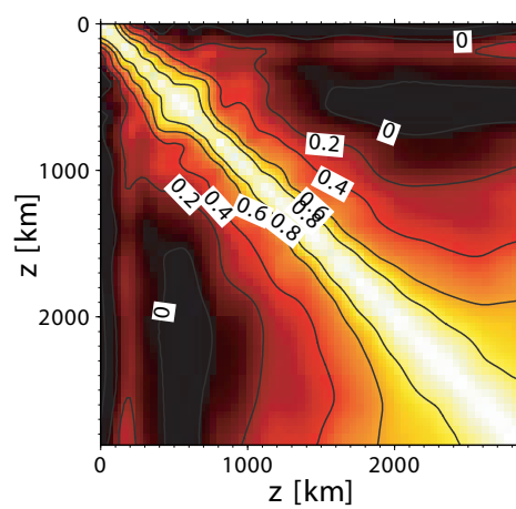
S20RTS
