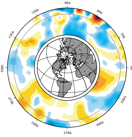
S20RTS
